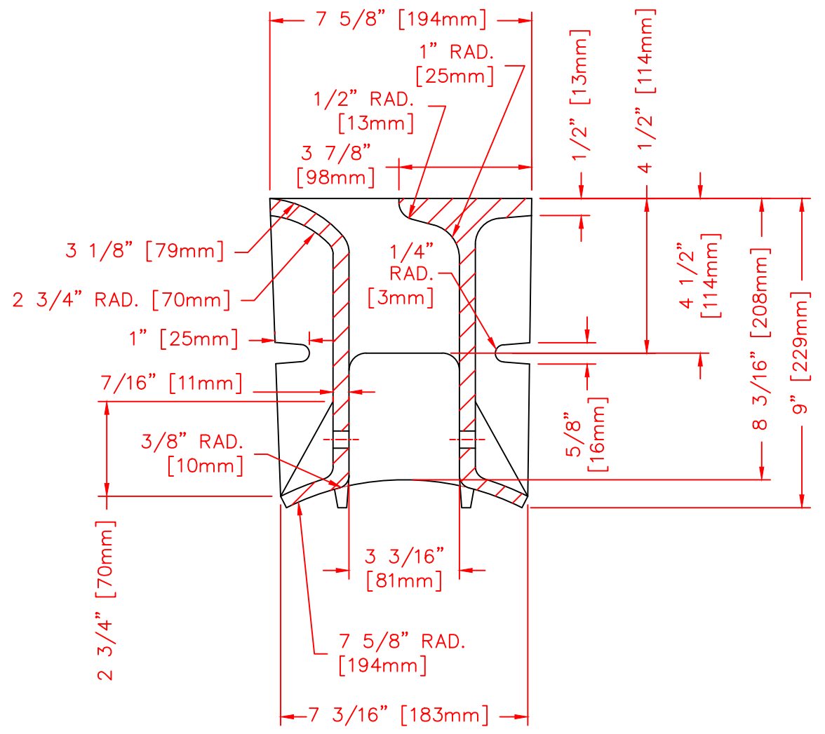
SECTION THRU VANE DRAIN HALF SCALE
