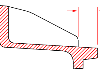
(4) GUSSETS 90° APART SECTION B-B
